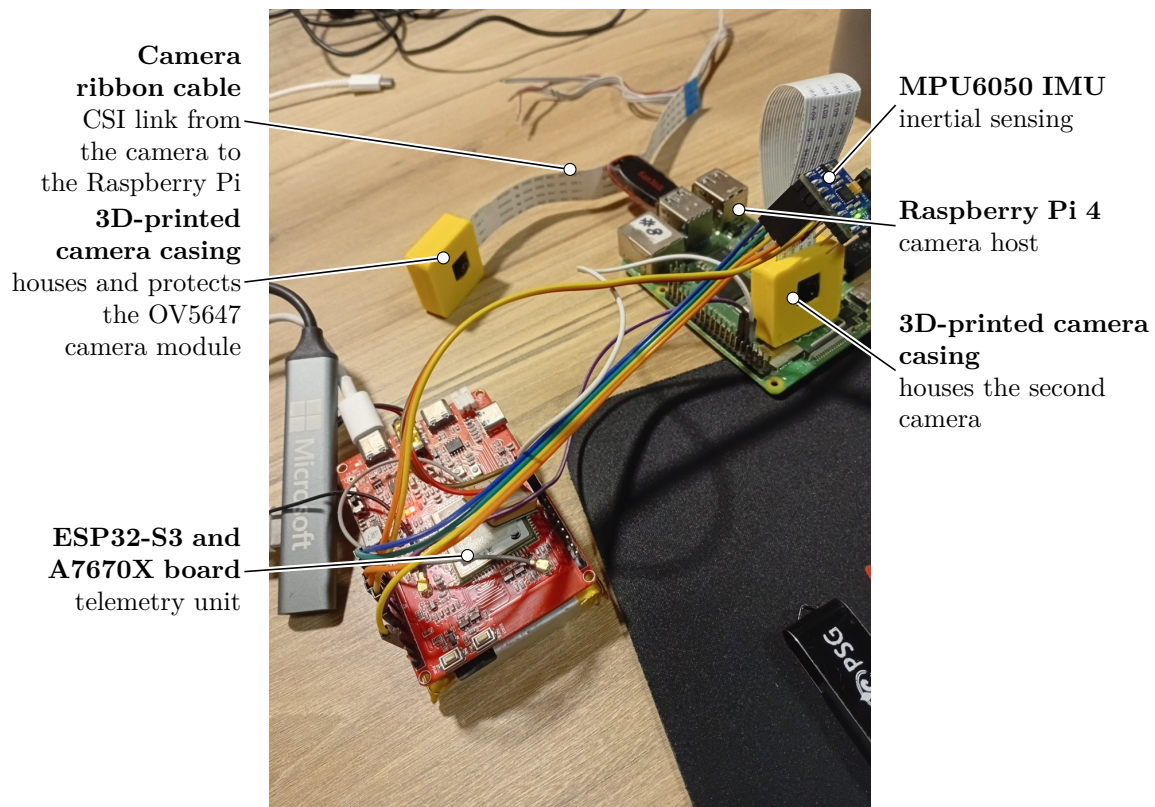
Figure 3.7: The cameras fitted in their 3D-printed casings, shown with the rest of the bench setup.
