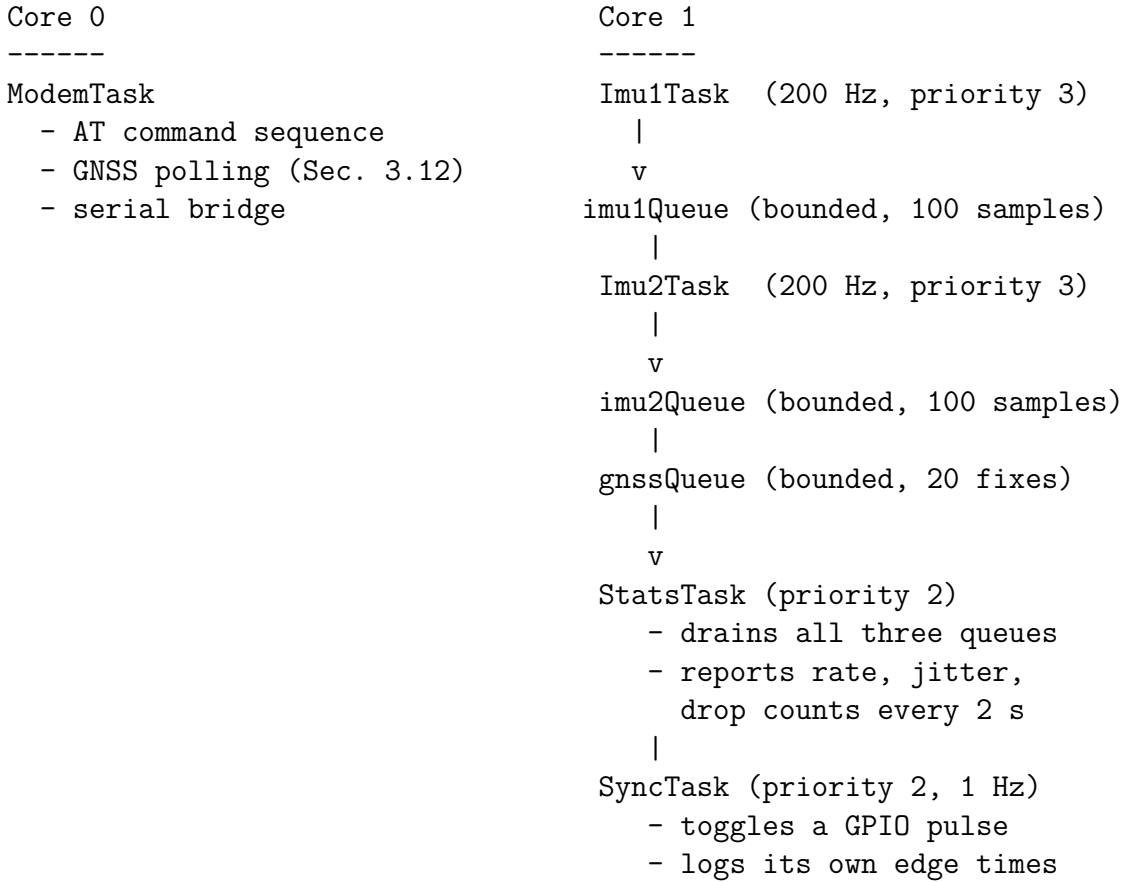
Figure 3.2: Task and queue architecture, firmware v0.4.0.
