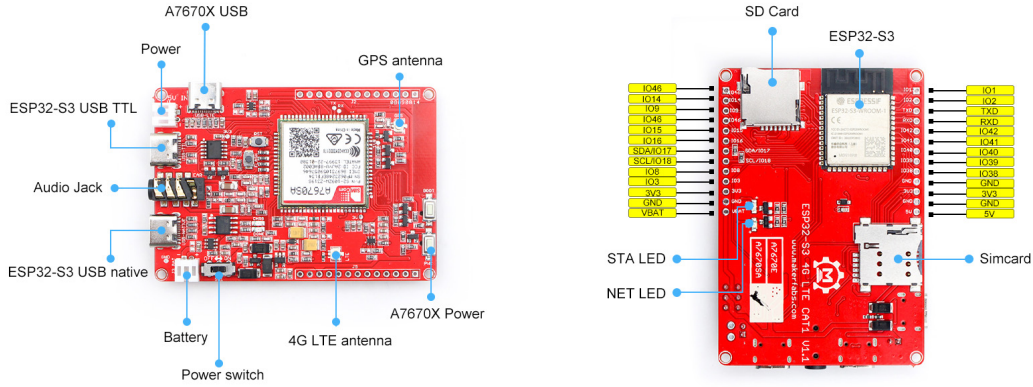
Figure 3.1: Makerfabs ESP32-S3 4G LTE CAT1 A7670X board: manufacturer-labelled ports (left) and pinout (right) [59].
