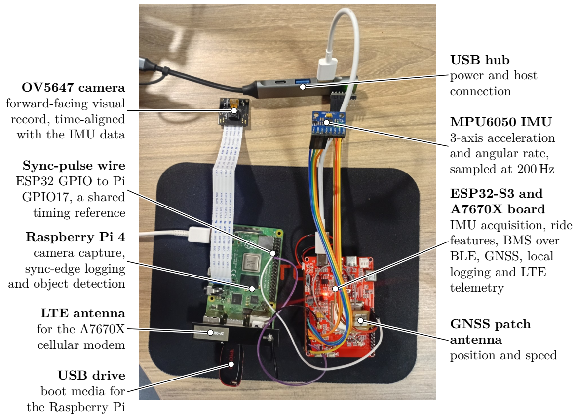
Figure 3.5: Bench setup of the telemetry system, with each component labelled by its role.
