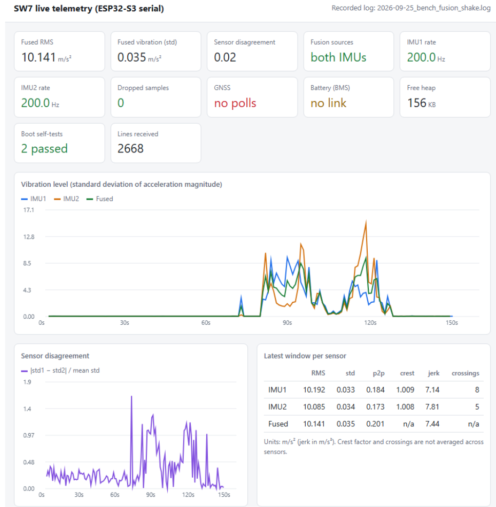
Figure 3.4: A 150-second bench session recorded from power-up and replayed through the dashboard: still until about 75 s, disturbed by hand until about 128 s, then still again.
